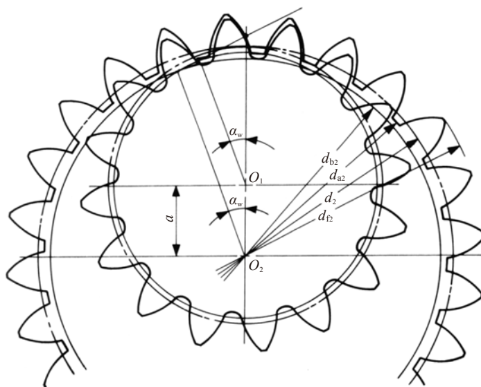
图 4.4 内齿轮与正齿轮的啮合 ( \alpha = 20^\circ , z_1 = 16 , z_2 = 24 , x_1 = x_2 = +0.5 )
