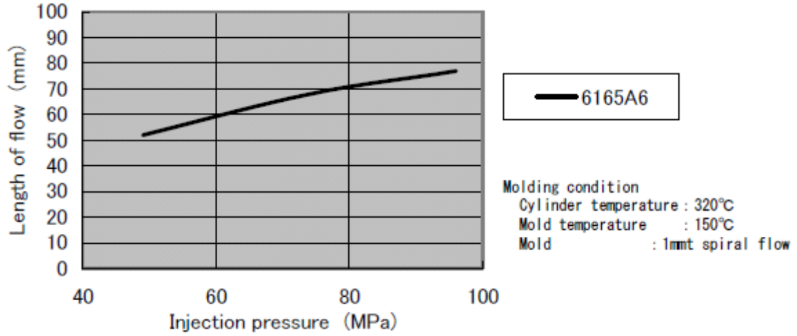
(Figure 3-1) Flowability(1mmt)
